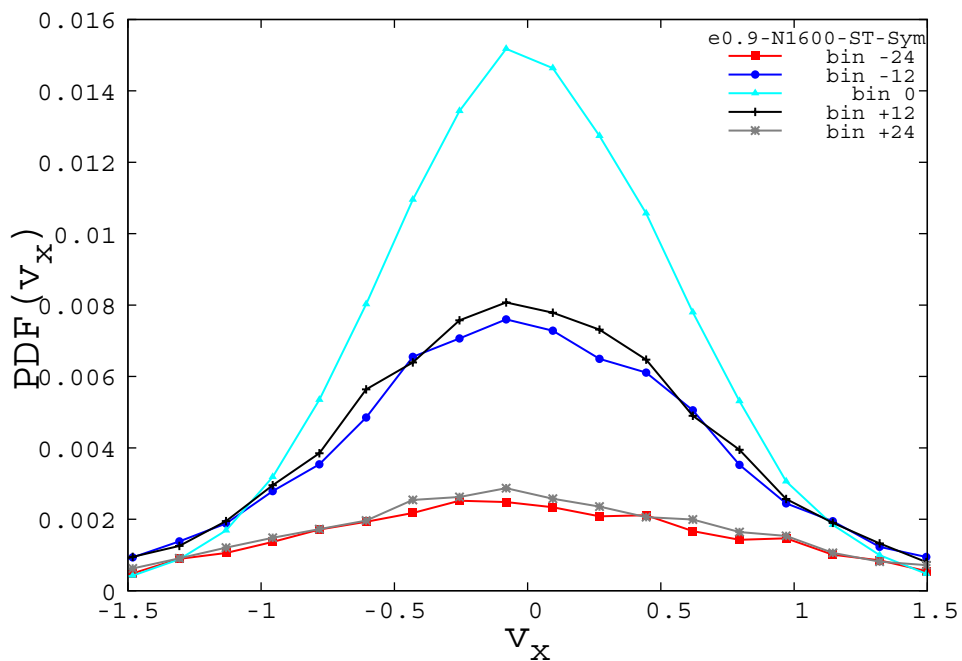
Figure 2.3 - 5: Simulations of granular gas in 3d rectangular cell
